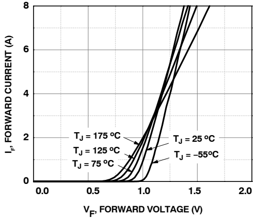
Figure 1. Forward Characteristics
