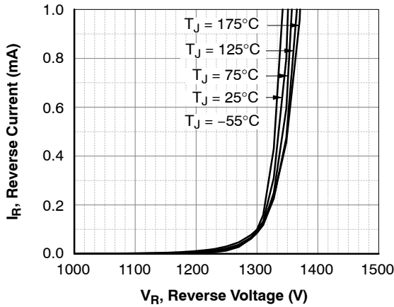
Figure 3. Reverse Characteristics
