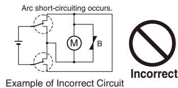
Example of Incorrect Circuit
