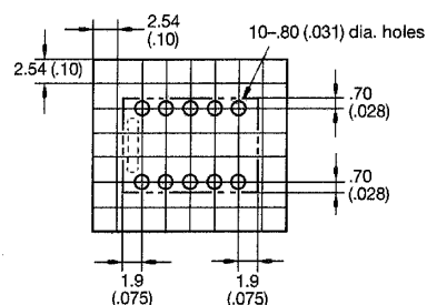
Mounting holes (Bottom view, dimensional tolerance ±0.1)
