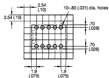
Mounting holes (Top view)
