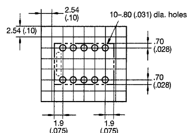
Mounting holes (Bottom view, dimensional tolerance ±0.1)
