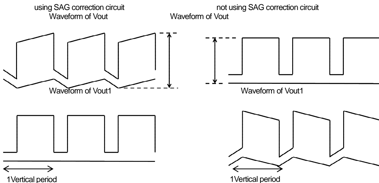
Waveform of Vout terminal and Vout1 terminal
