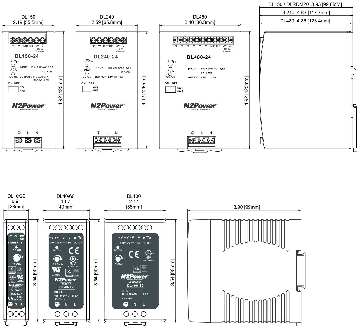
Figure 4-2 DL Dimensions
