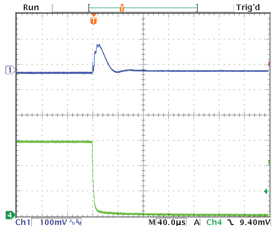
Step Load Transient Response (Vin=12V, Vout=3.3V, Load=12x10µF X5R 0805 ceramic, total 120µF, Iout=3A to 0A) Top trace=Vout, Bottom trace=Iout
