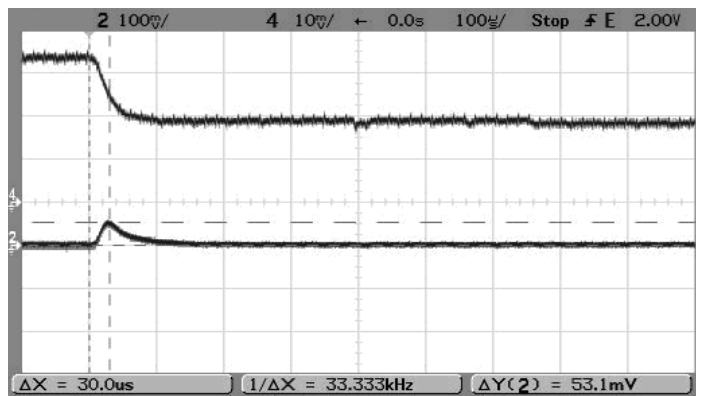
Trace 2=Vout, 100 mV/div. Trace 4=Iout, 1A/div.
