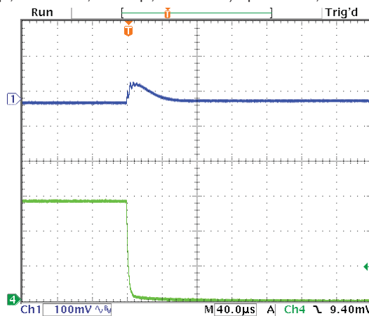
Step Load Transient Response (Vin=12V, Vout=5V, Cload=10x10µF X5R 0805 ceramic, plus 1x470µF, 7mΩ POSCAP, total 570µF, Iout=3A to 0A) Top trace=Vout, Bottom trace=Iout
