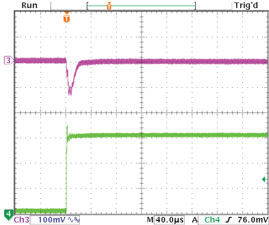
Step Load Transient Response (Vin=5.5V, Vout=3.3V, Load=5x10µF X5R 0805 ceramic, total 50µF, Iout=0A to 3A) Top trace=Vout, Bottom trace=Iout
