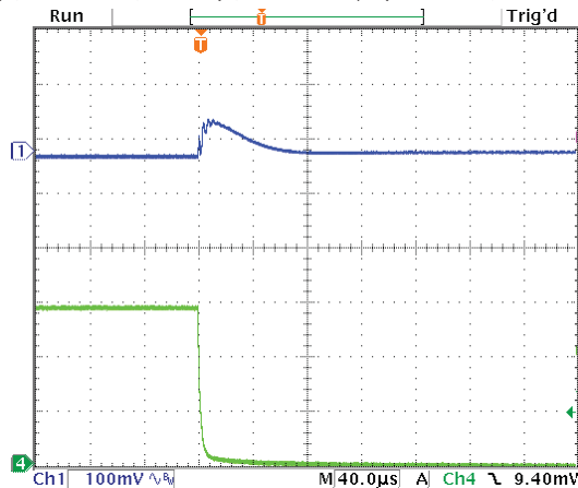
Step Load Transient Response (Vin=12V, Vout=1.8V, Cload=10x10µF X5R 0805 ceramic, plus 1x470µF, 7mΩ POSCAP, total 570µF, Iout=3A to 0A) Top trace=Vout, Bottom trace=Iout
