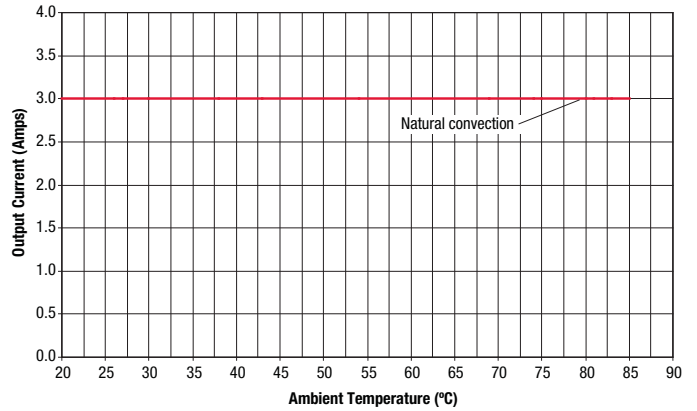
Maximum Current Temperature Derating @ Sea Level ( V_{IN} = 7V and 12V , V_{OUT} = 5V and 6V )
