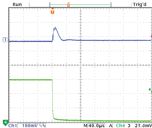
Step Load Transient Response (Vin=4.5V, Vout=1.8V, Cload=10x10µF X5R 0805 ceramic, plus 1x470µF, 7mΩ POSCAP, total 570µF, Iout=3A to 0A) Top trace=Vout, Bottom trace=Iout
