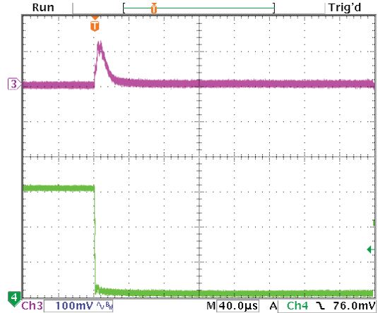
Step Load Transient Response (Vin=5.5V, Vout=3.3V, Load=5x10µF X5R 0805 ceramic, total 50µF, Iout=3A to 0A) Top trace=Vout, Bottom trace=Iout
