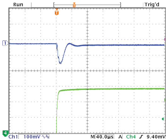
Step Load Transient Response (Vin=12V, Vout=3.3V, Load=12x10µF X5R 0805 ceramic, total 120µF, Iout=0A to 3A) Top trace=Vout, Bottom trace=Iout
