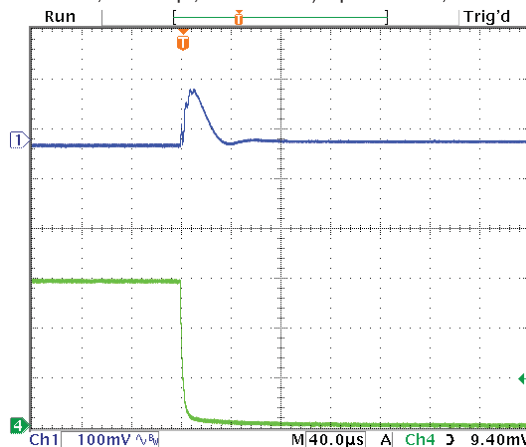
Step Load Transient Response (Vin=7.5V, Vout=5V, Cload=10x10µF X5R 0805 ceramic, plus 1x470µF, 7mΩ POSCAP, total 570µF, Iout=3A to 0A) Top trace=Vout, Bottom trace=Iout
