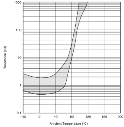
Resistance-Temperature Charac. Range
