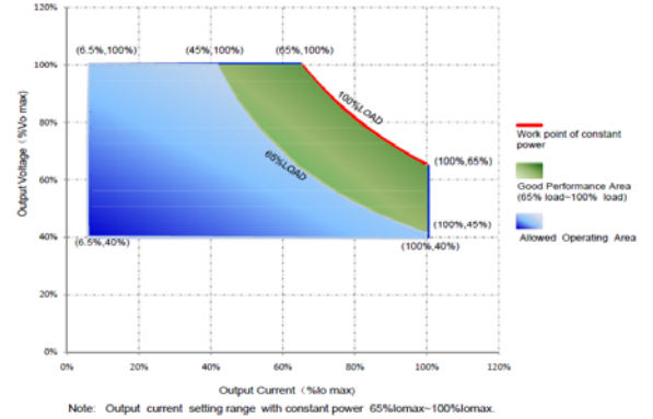
V/I Operating Area
