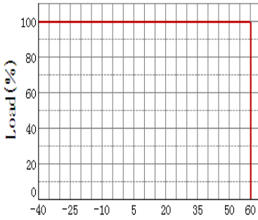
Derating Curve
