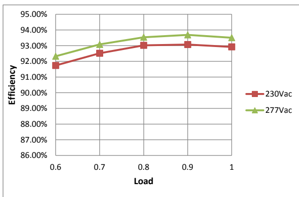
Efficiency VS. Load Curve (Io=4000mA)
