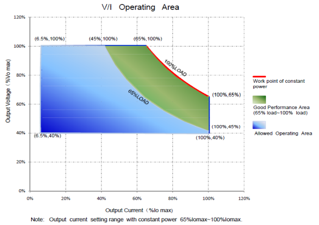
V/I Curve
