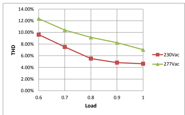
THD Curve
