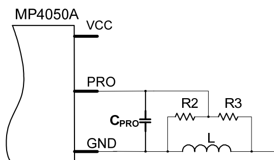
Figure 8: Decoupling Capacitor
