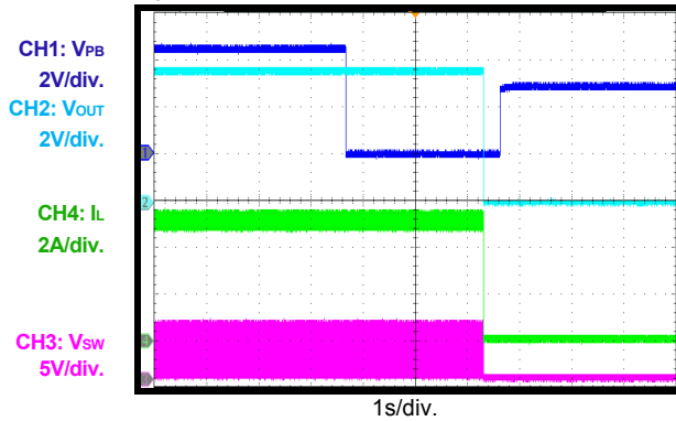
Power Off by PB Pin, BOOST Mode V_{BATT}=3.7V , V_{OUT}=5V , R_{OLIMIT}=71.5k\Omega , I_{LOAD}=3A
