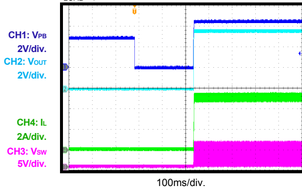
Power On by PB Pin, BOOST Mode V_{BATT}=3.7V , V_{OUT}=5V , R_{OLIMIT}=71.5k\Omega , I_{LOAD}=3A
