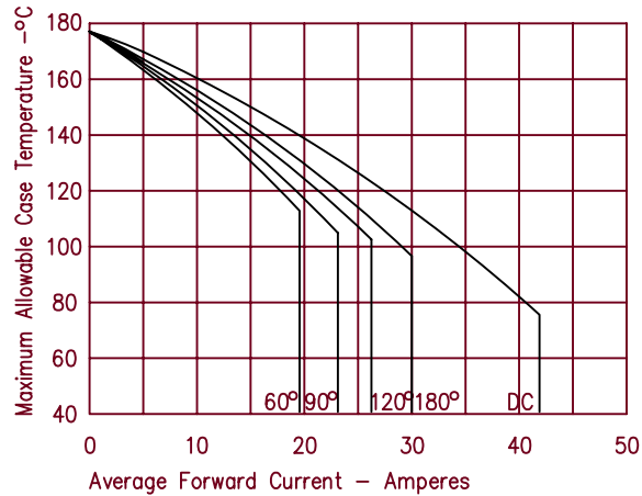
Figure 5 Forward Current Derating – Reverse Polarity – Per Leg
