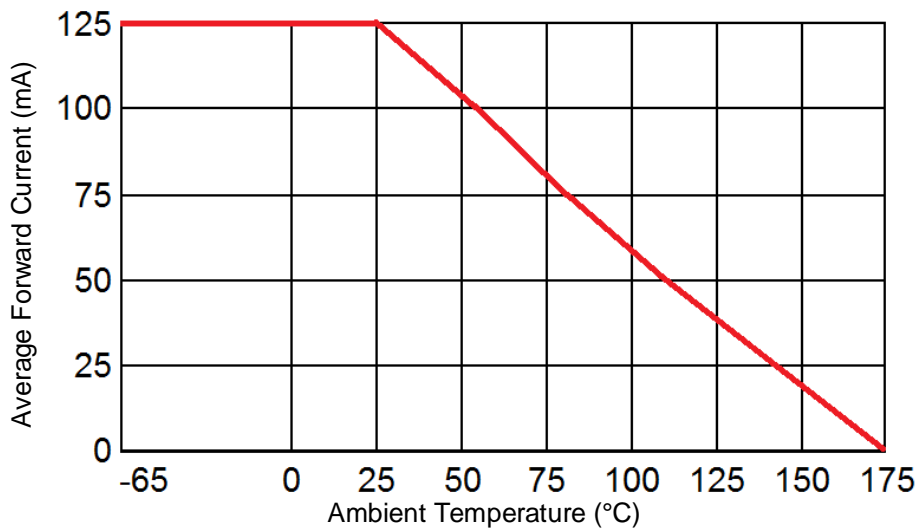
FIGURE 2 1N5181 - 1N5184
