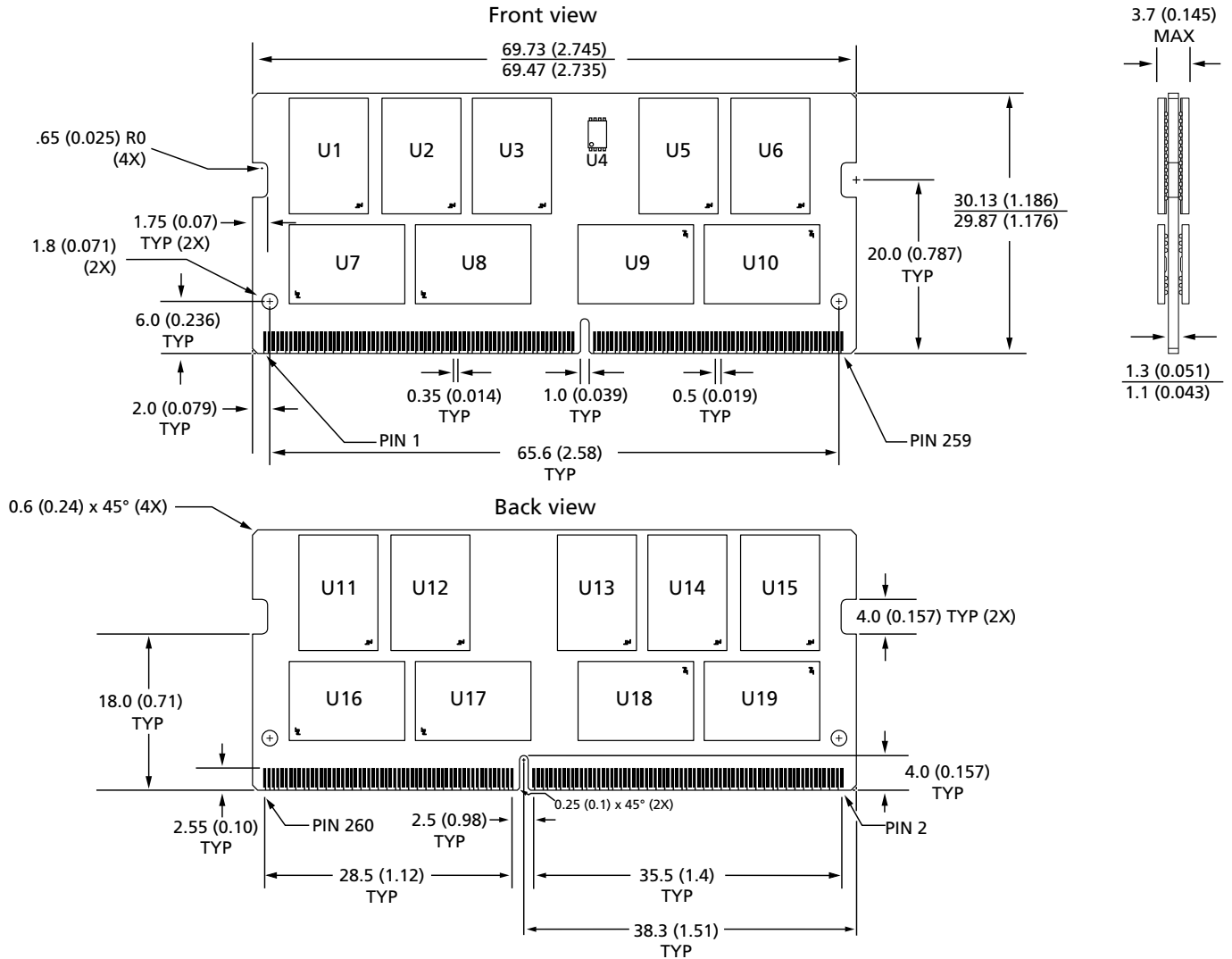
Figure 5: 260-Pin DDR4 SODIMM, R/C-H (PCB 1813)
