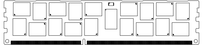
Figure 2: 240-Pin RDIMM (MO-269 R/C E2)
