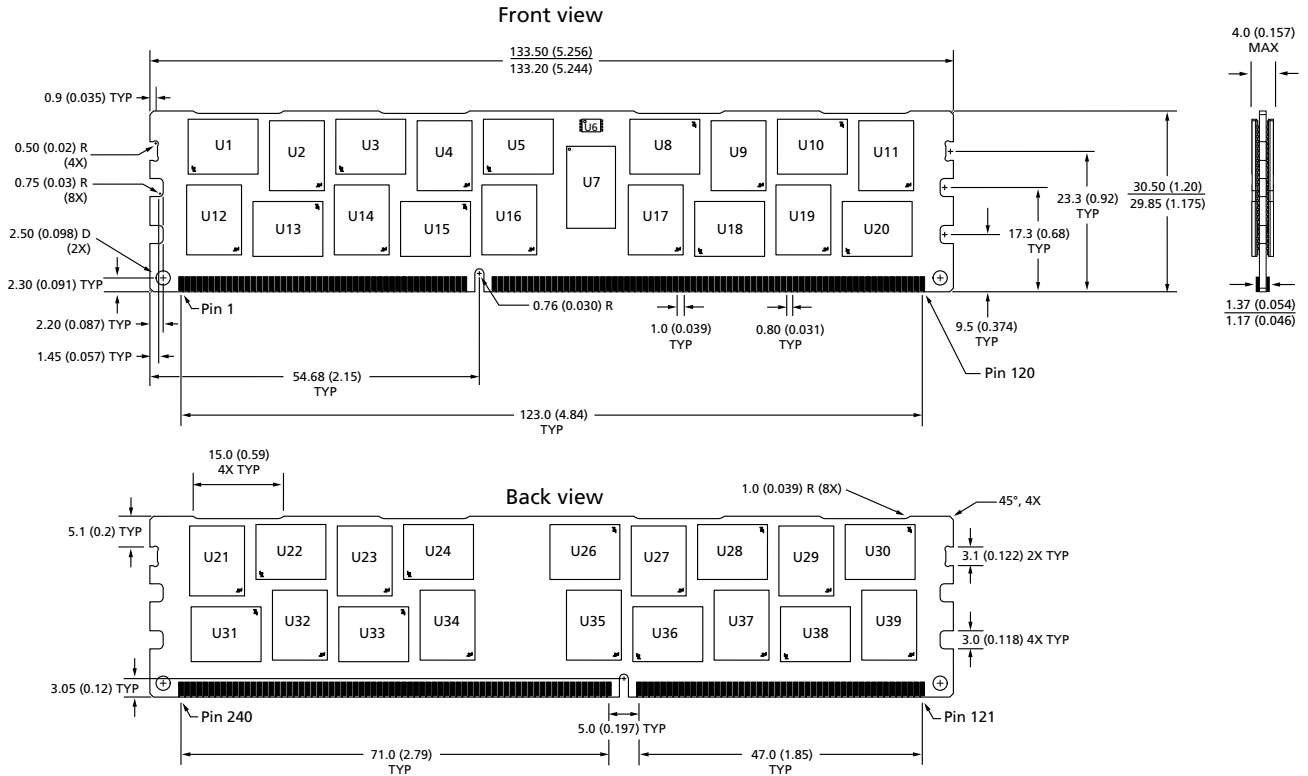
Figure 6: 240-Pin DDR3 RDIMM (PCB 1354, R/C-E2)
