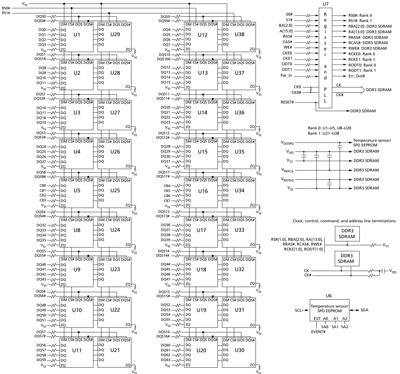
Figure 3: Functional Block Diagram (PCB 0757, R/C-J)
