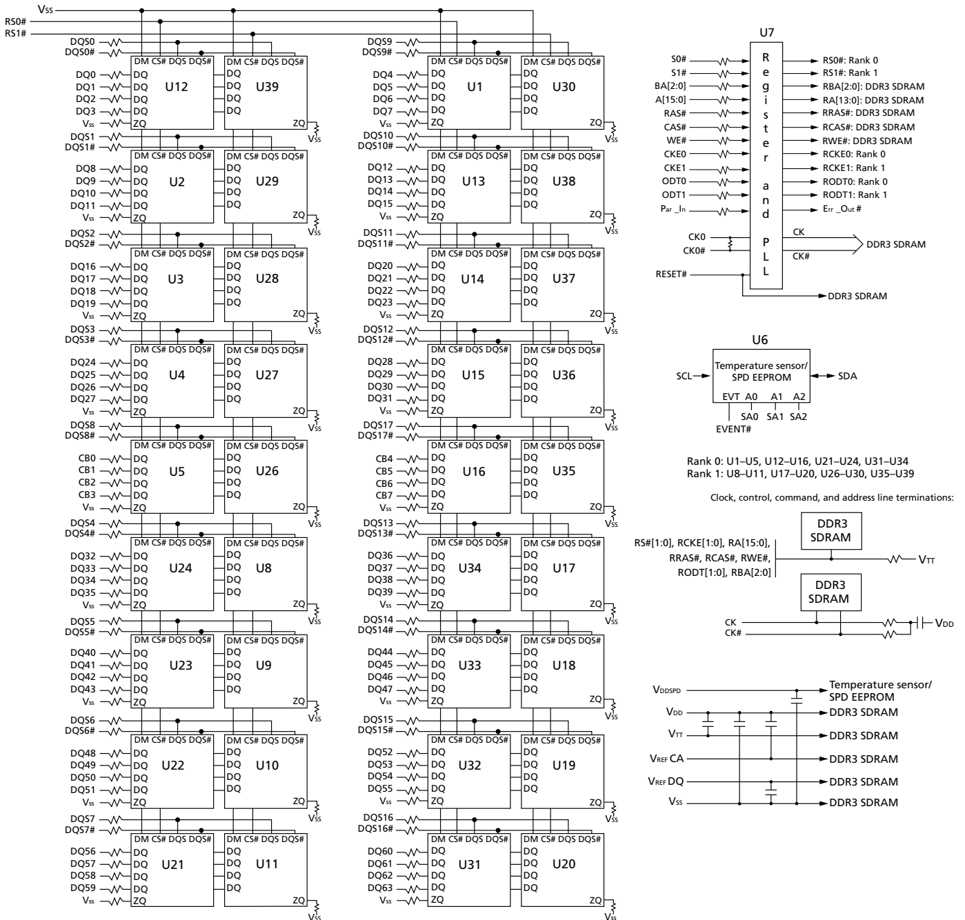
Figure 4: Functional Block Diagram (PCB 1354, R/C-E2)
