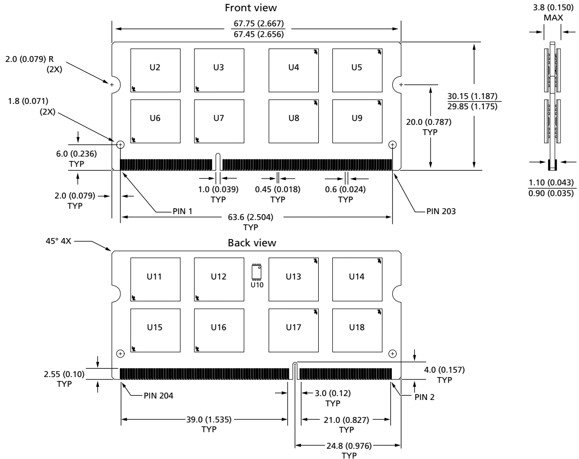
Figure 5: 204-Pin DDR3 SODIMM (PCB 1569, R/C-F3)
