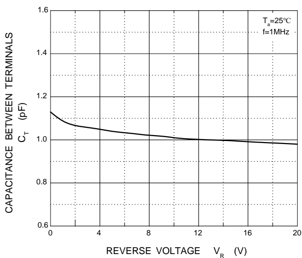
Fig. 5 Capacitance Characteristics
