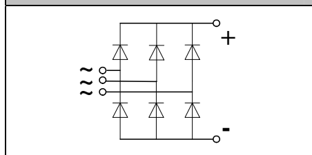
Circuit
