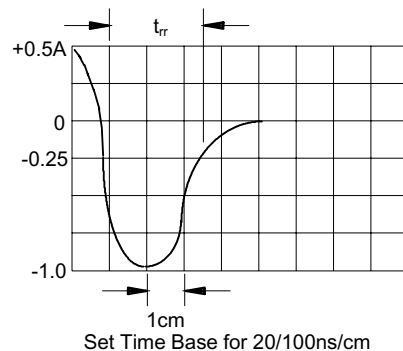
Set Time Base for 20/100ns/cm
