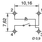
Single LED
