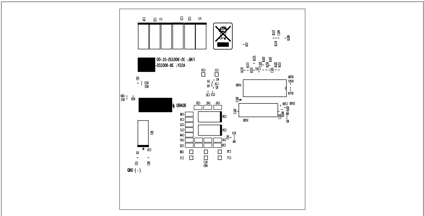
Bottom Silkscreen
