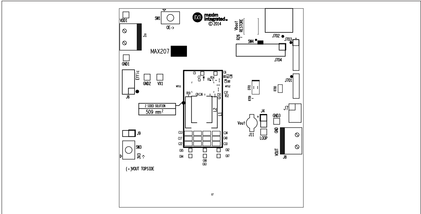
Top Silkscreen
