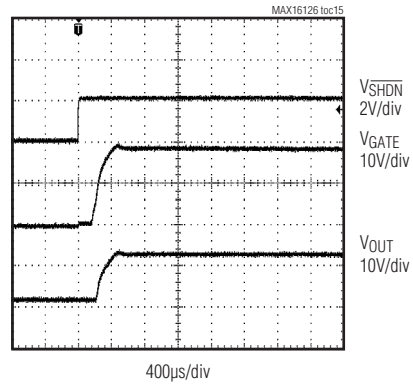
OVERVOLTAGE LIMITER ( V_{OV} = 4V , V_{QV} = 20V , C_{IN} = 0.1\mu F , C_{OUT} = 100\mu F )
