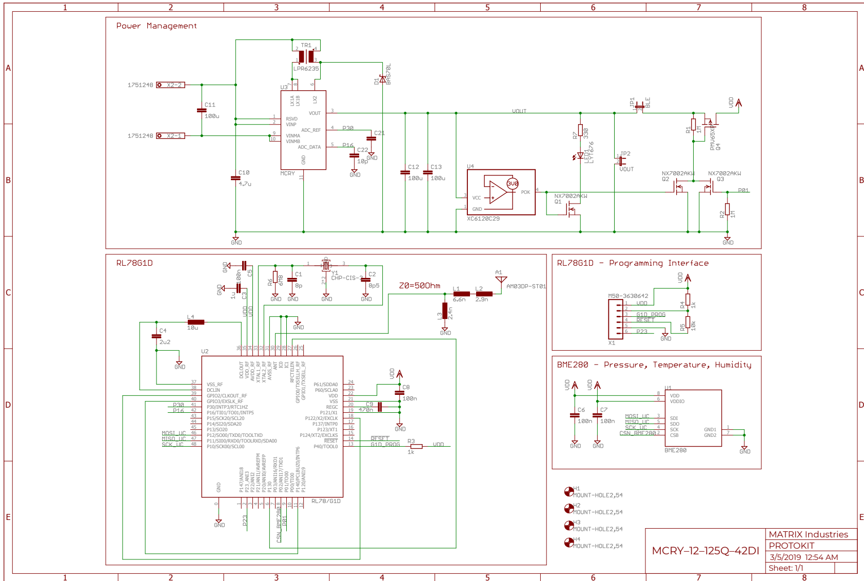
Figure 6: MCRY-PROTOKIT Schematics
