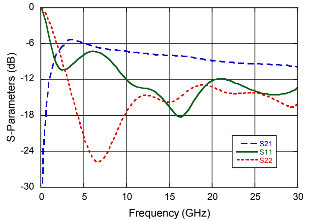
S-Parameters V_{C1} = -0.2 V, V_{C2} = -2.0 V
