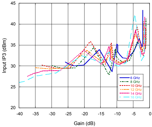
Input IP3 vs. Attenuation, SCL P_{IN} = 6\text{ dBm}
