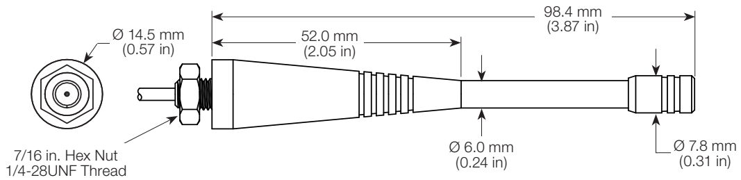
Figure 7. PW LTE Band 13 Antenna Dimensions
