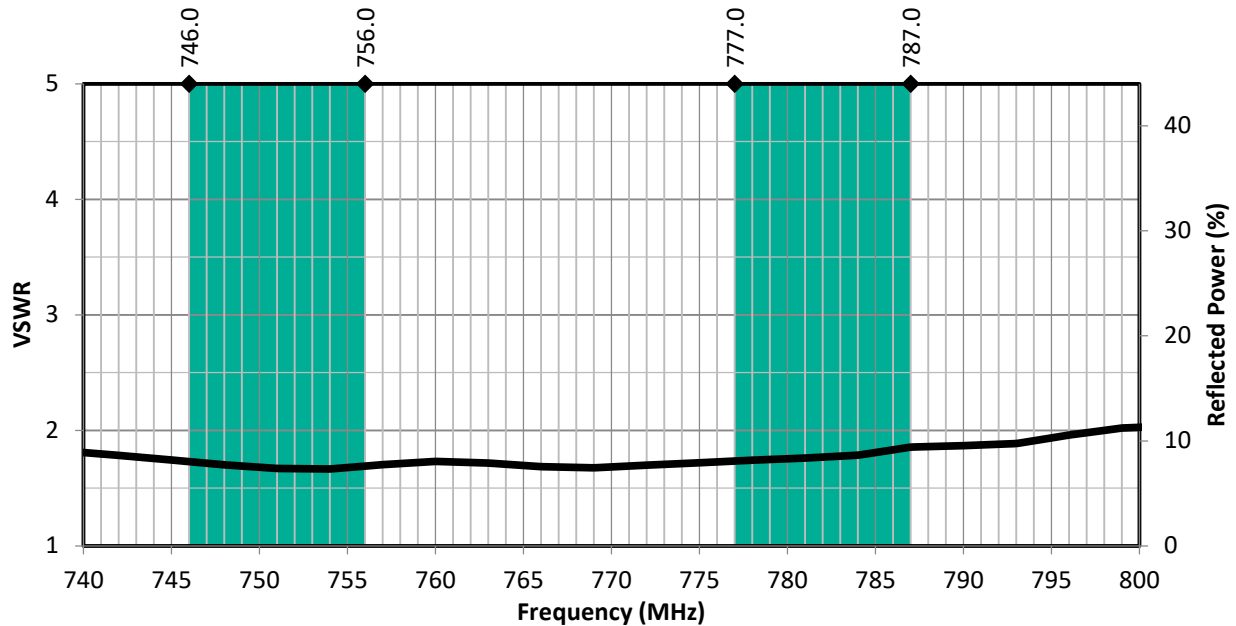
Figure 1. PW LTE Band 13 Antenna VSWR with Band 13 Uplink/Downlink Highlights
