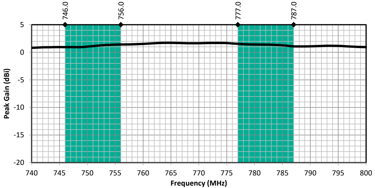
Figure 4. PW LTE Band 13 Antenna Peak Gain with Band 13 Uplink/Downlink Highlights
