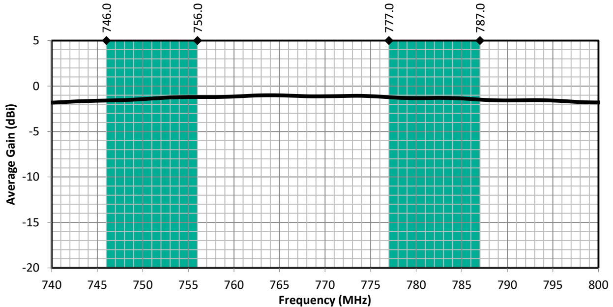
Figure 5. PW LTE Band 13 Antenna Average Gain with Band 13 Uplink/Downlink Highlights
