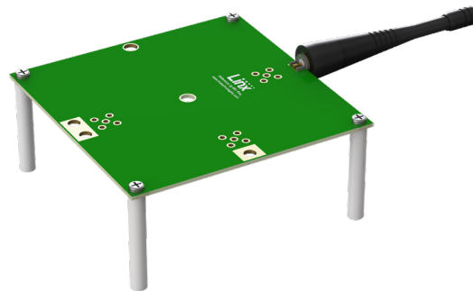
Figure 8. PW LTE Band 13 Antenna Shown On Edge of Evaluation Board
