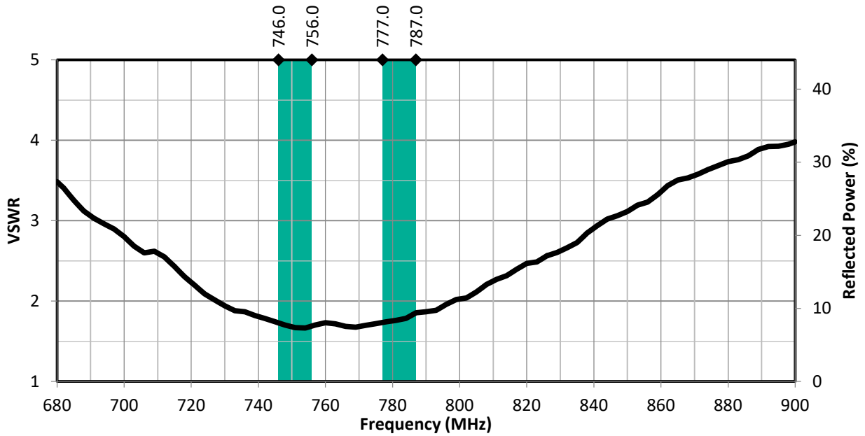
Figure2. PW LTE Band 13 Antenna Full Bandwidth VSWR
