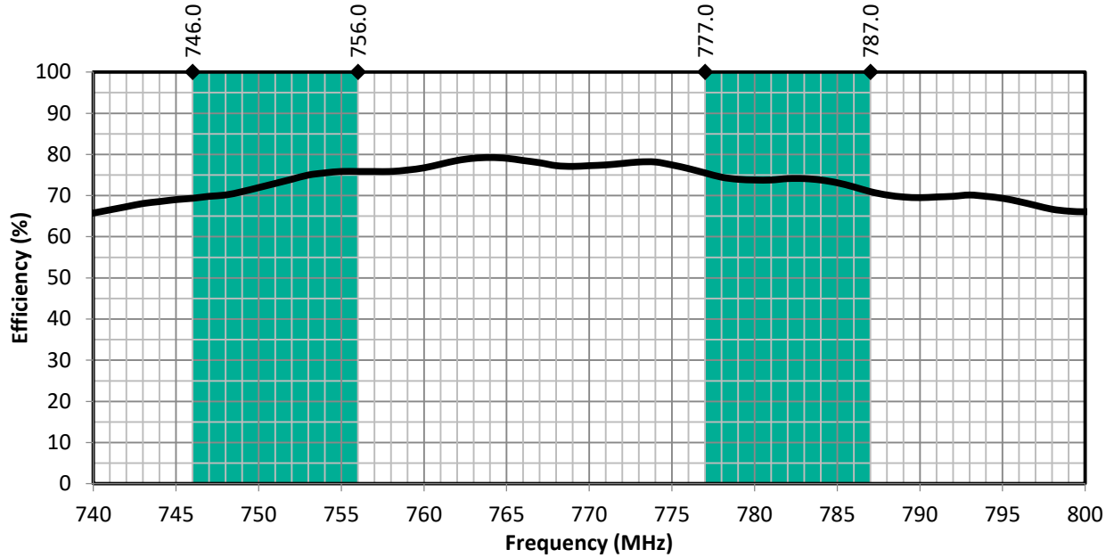
Figure 6. PW LTE Band 13 Antenna Radiation Efficiency with Band 13 Uplink/Downlink Highlights
