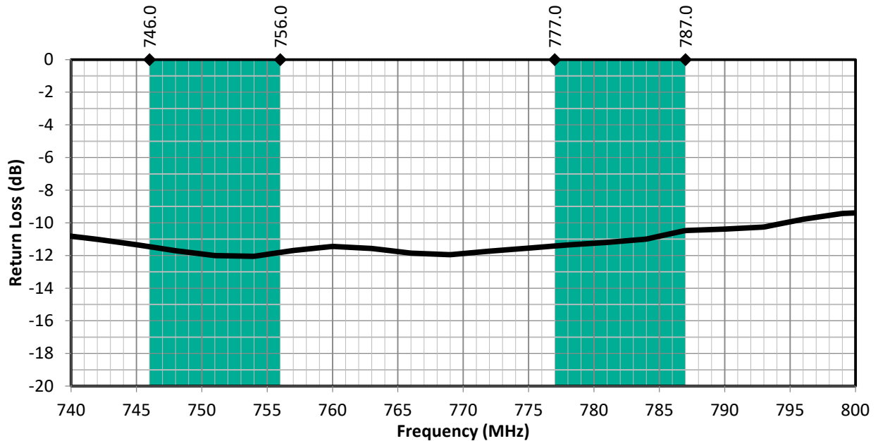
Figure3. PW LTE Band 13 Antenna Return Loss with Band 13 Uplink/Downlink Highlights
