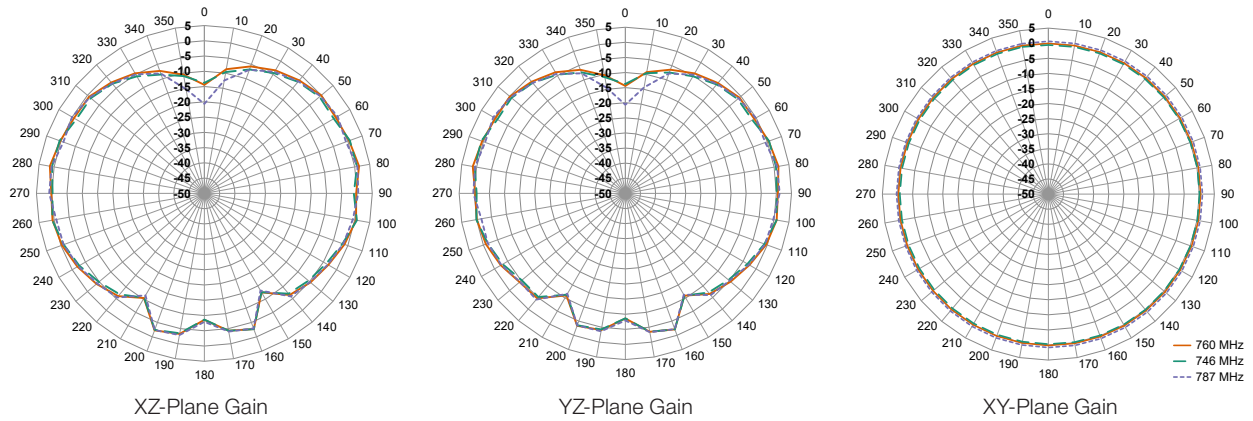
Figure9. Radiation Patterns for PW LTE Band 13 Antenna
