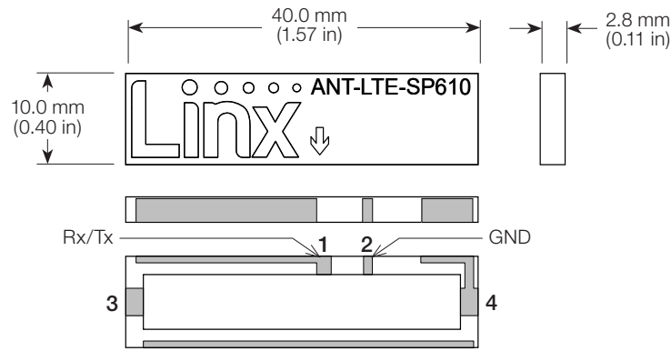
Figure 6. SP610 Dimensions
