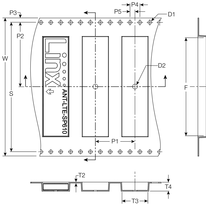
Figure 12. Tape Specifications for the SP610 Antenna
