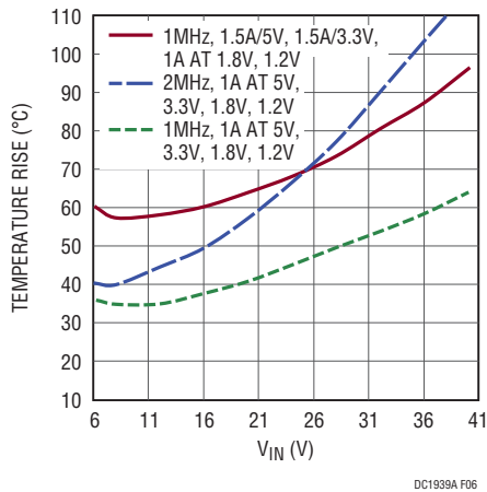
Figure 6. LT8602 Case Temperature Rise, T_A = 25^\circ C
