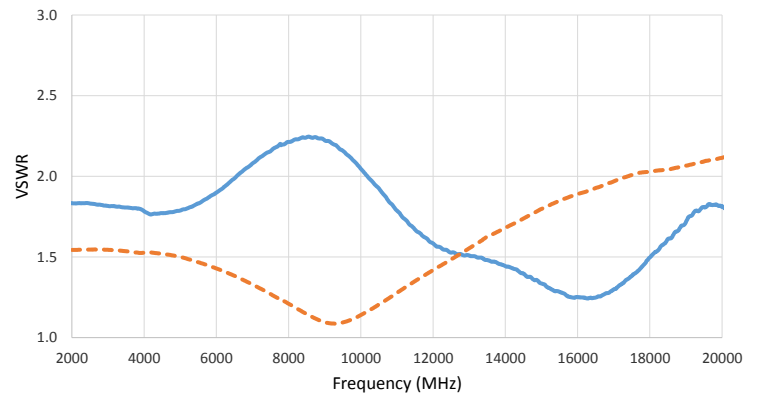
Input (Solid) and Output VSWR (Dashed)
