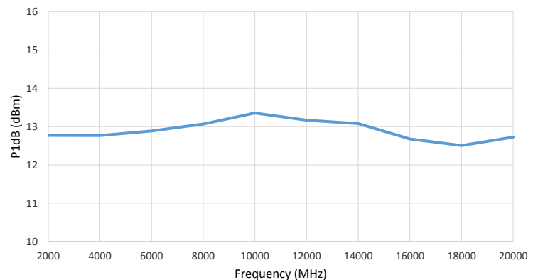
Power Out @ 1dB Compression
