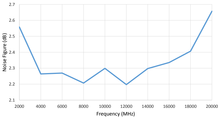
Noise Figure
