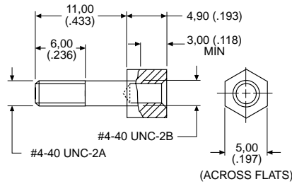
Jackpost
