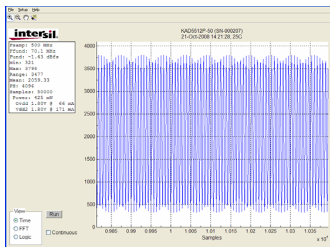
FIGURE 2. TIME-DOMAIN DISPLAY
