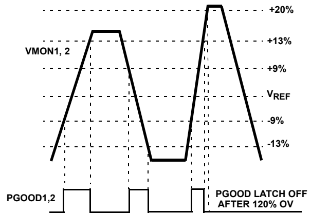
FIGURE 17. POWER-GOOD THRESHOLD WINDOW
