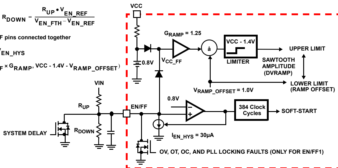
FIGURE 13. SIMPLIFIED ENABLE AND VOLTAGE FEEDFORWARD CIRCUIT
