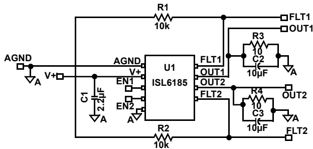
FIGURE 32A. ISL6185xEVAL SCHEMATIC
