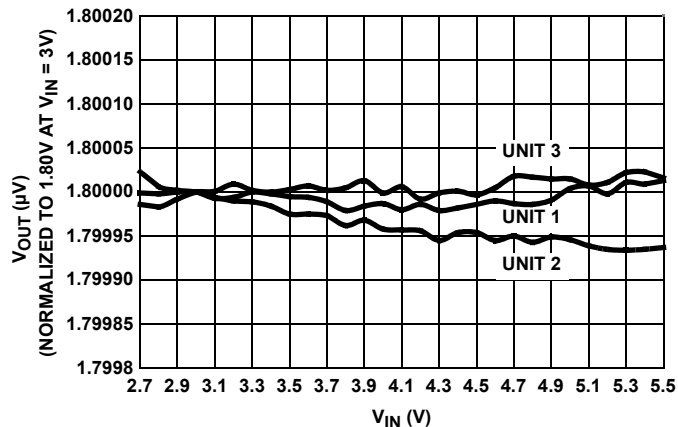
FIGURE 45. LINE REGULATION (3 REPRESENTATIVE UNITS)
