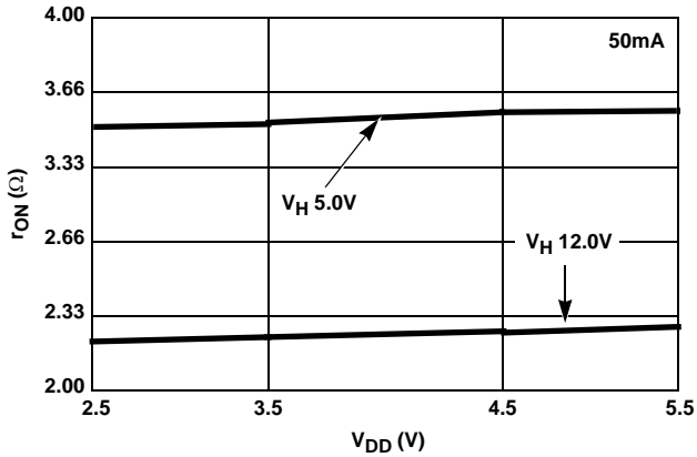
FIGURE 5. r_{ON} vs V_{DD} SOURCE RESISTANCE
