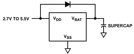
FIGURE 24. SUPERCAPACITOR CHARGING CIRCUIT
