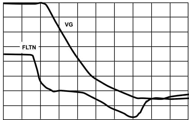
VOLTAGE (2V/DIV) TIME (1µs/DIV) FLT N = 0.001µF
