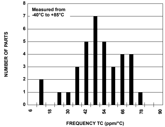
FIGURE 2. FREQUENCY DRIFT WITH TEMPERATURE
