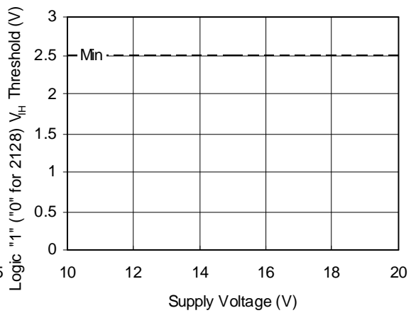
Figure 13B. Logic "1" ("0" for 2128) V_{IH} Threshold vs. Voltage
