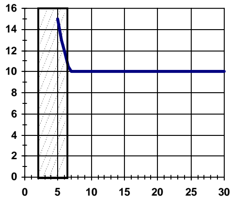
Figure 9- R_{dsOn} (m \Omega ) vs V_{cc-Vin} (V)
