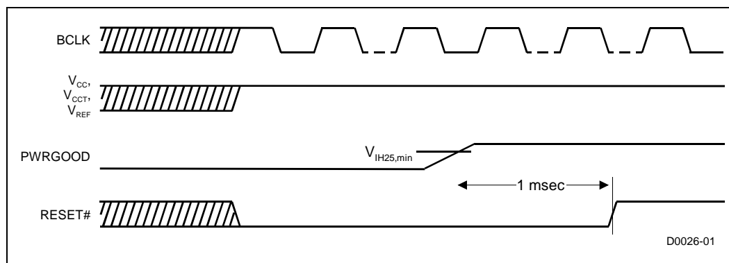
Figure 22. PWRGOOD Relationship at Power On
