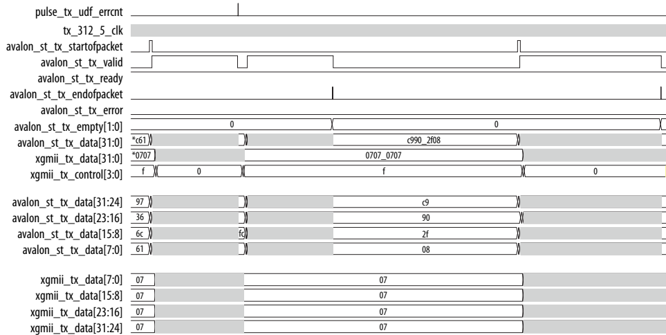
Figure 18. Error Condition—Underflow
