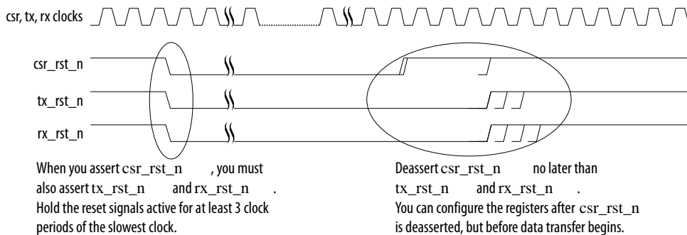
Figure 25. CSR Reset
