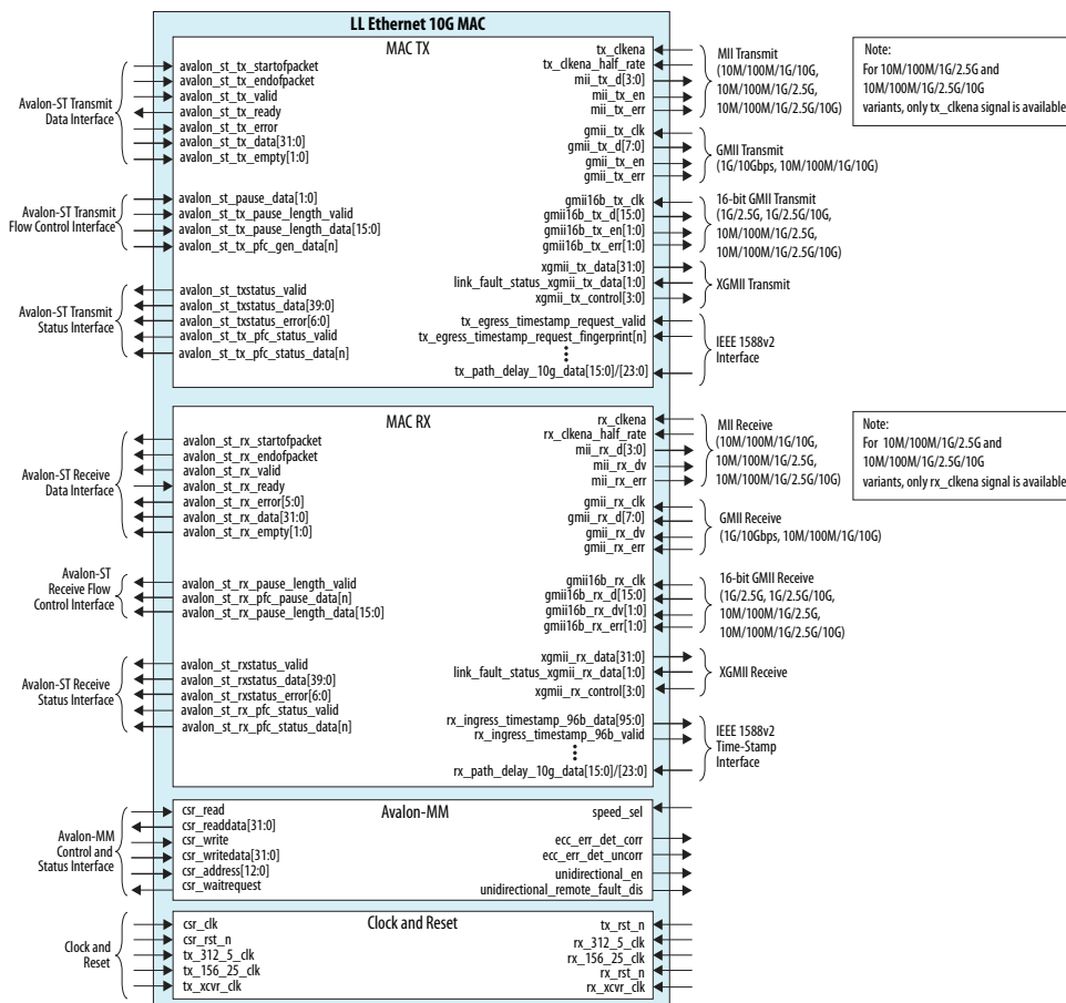
Figure 9. Interface Signals
