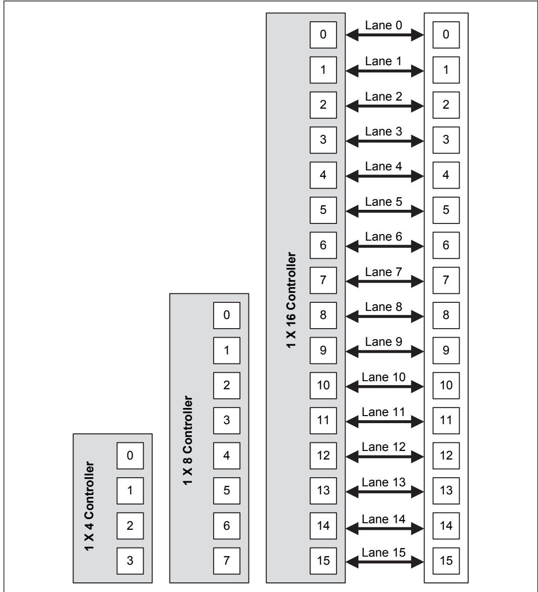
Figure 4. PCI Express* Typical Operation 16 Lanes Mapping
