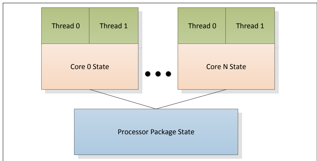
Figure 12. Idle Power Management Breakdown of the Processor Cores
