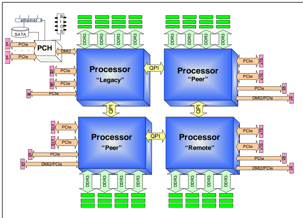
Figure 1-3. Intel Xeon Processor E5-4600 v2 Product Family on the 4 Socket Platform
