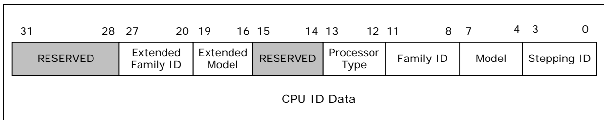
Figure 2-21. CPUID Data
