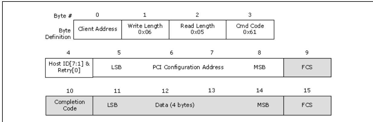
Figure 2-45. RdPCIFconfig()
