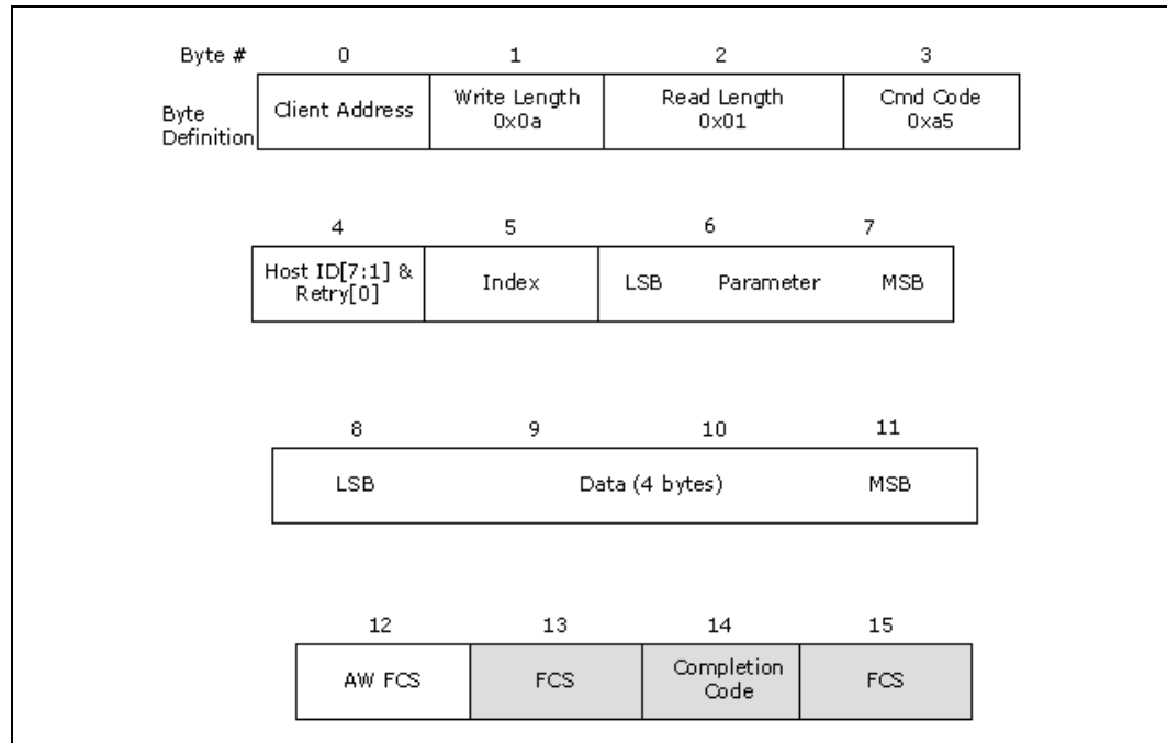
Figure 2-11. WrPkgConfig()
