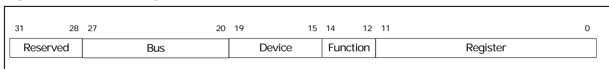
Figure 2-44. PCI Configuration Address
