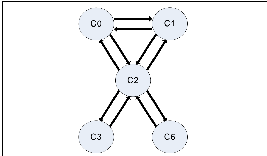
Figure 4-3. Package C-State Entry and Exit
