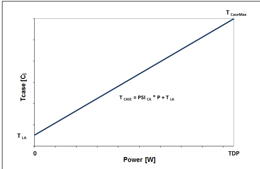
Figure 5-1. T_{Case} Temperature Thermal Profile
