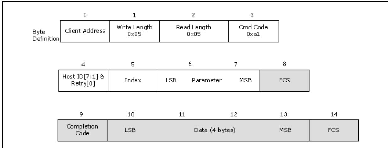
Figure 2-10. RdPkgConfig()
