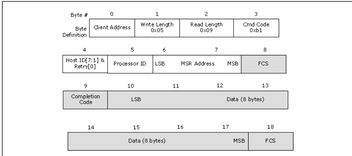
Figure 2-43. RdIAMSRO
