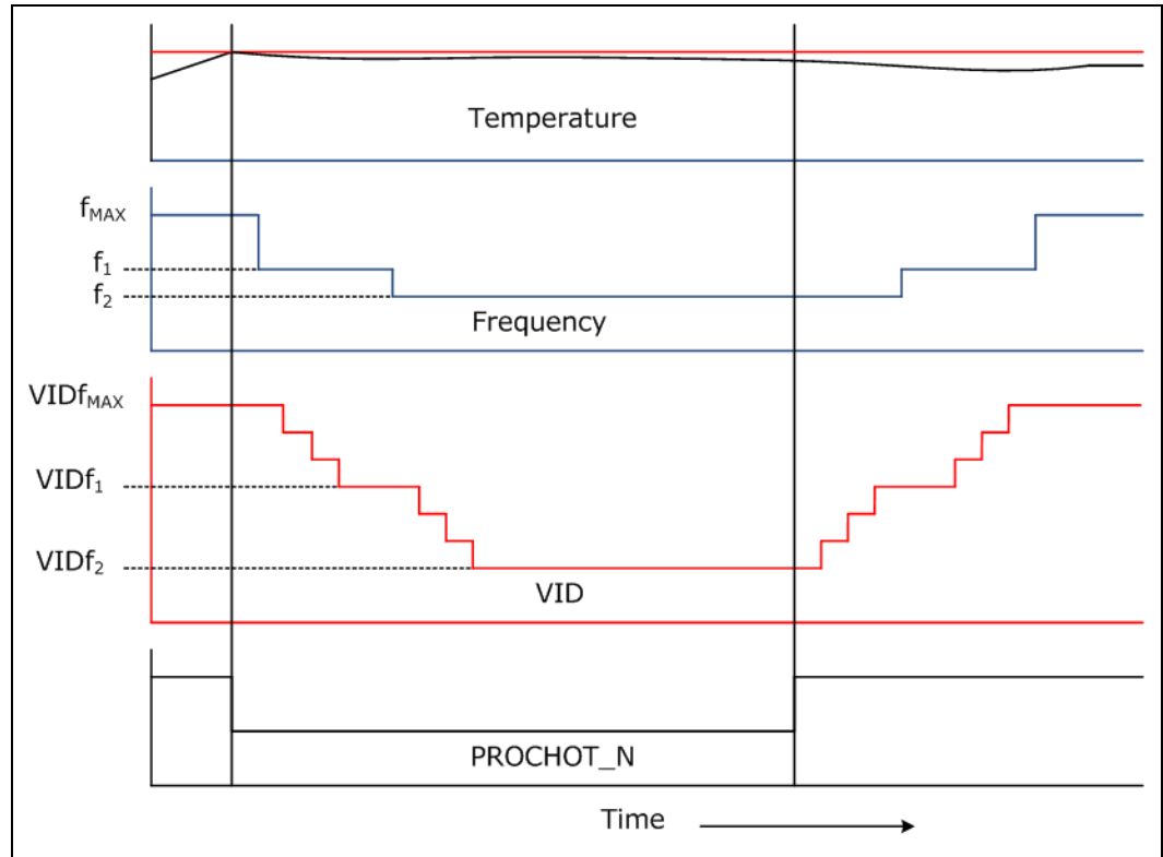
Figure 5-6. Frequency and Voltage Ordering
