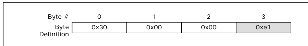
Figure 2-4. Ping() Example
