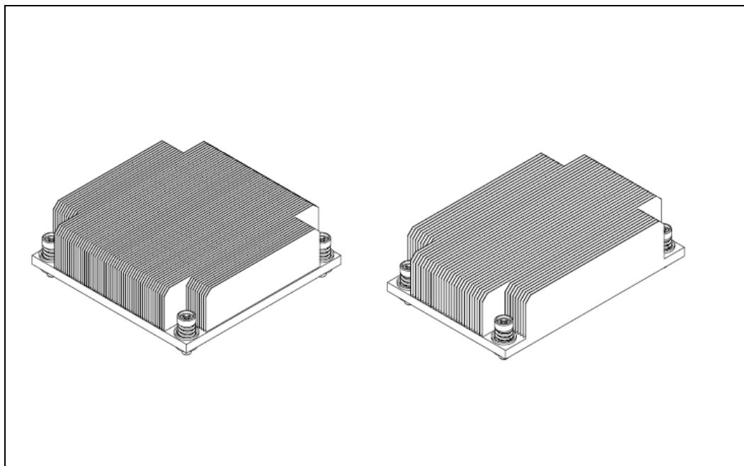
Figure 10-3. STS200P and STS200PNRW 25.5 mm Tall Passive Heat Sinks
