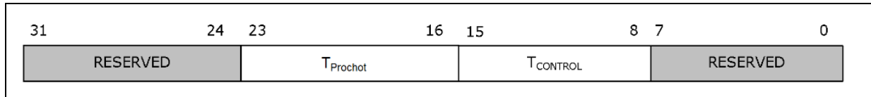
Figure 2-30. Temperature Target Read
