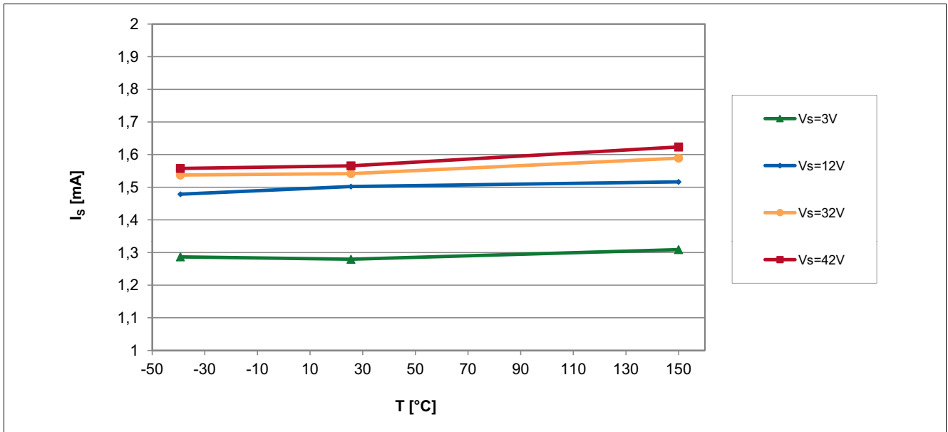
Figure 6-3 Supply Current of the TLE4968-1K over Temperature
