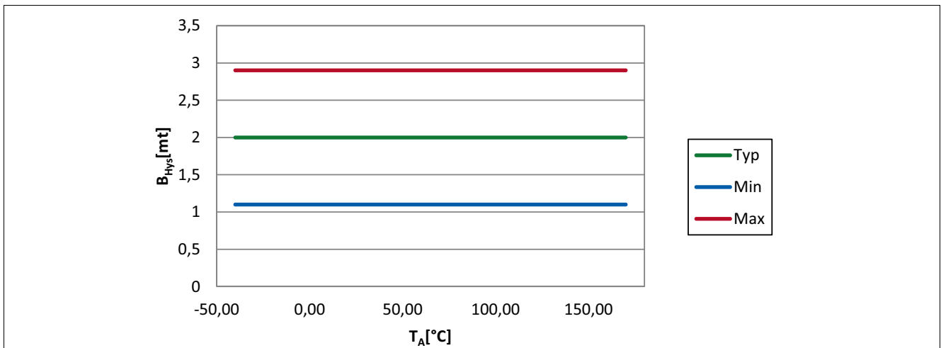
Figure 5-3 Hysteresis (B Hys ) of the TLE4968-1K over Temperature
