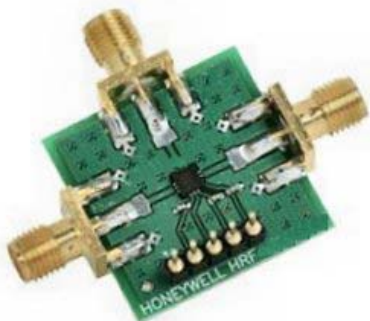
HRF-SW1000 Evaluation Board
