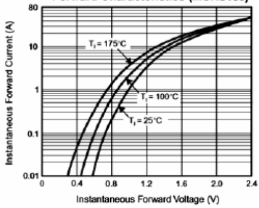
Fig. 3 – Typical Instantaneous Forward Characteristics (MURS160)
