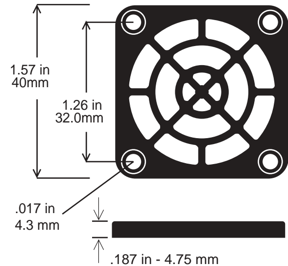
SC40-P10 Guard
