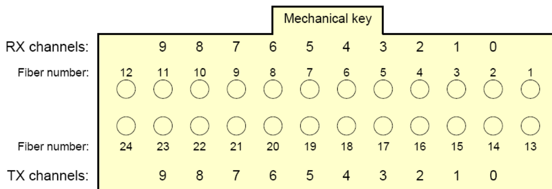
Figure 3. Optical Lane Assignment (View from the front, looking into the MPO receptacle)
