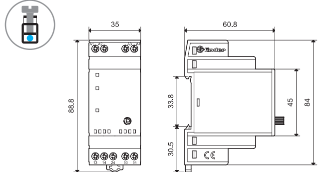
Type 19.42 Screw terminal
